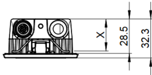
Figure 6: Dimensions – Side view (height)
