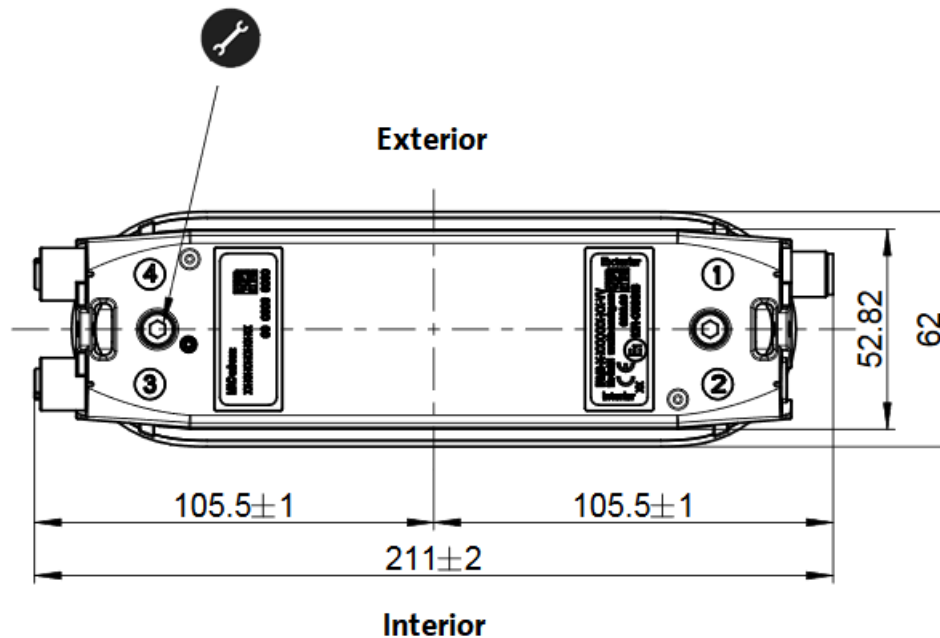
Figure 5: Dimensions – bottom view (all measures in mm)
