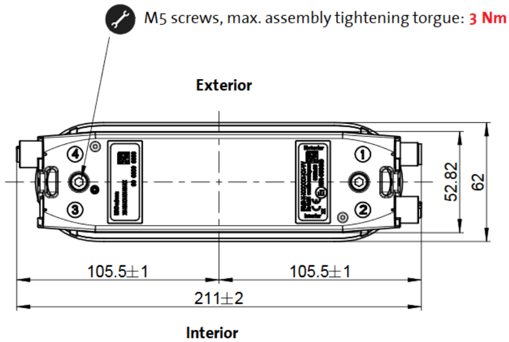
Figure 6: Dimensions – Bottom view IRMA6-SENSOR-HD-00-ETH-IO-00
