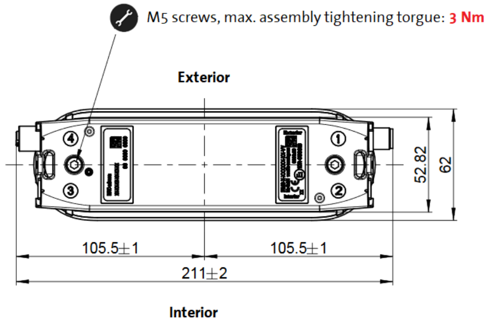
Figure 5: Dimensions – Bottom view: IRMA6-SENSOR-HD-00-ETH-00-R
