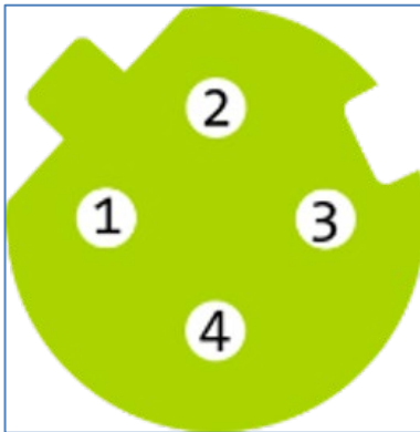
M12 Ethernet (female, d-coded)
